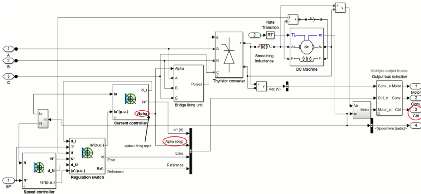
Location of the Firing Angle Signal Inside the Ctrl Output Vector
